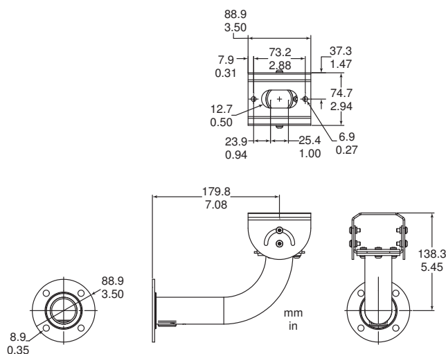
LTC 9215/00S Korte Wandmontagebeugel
