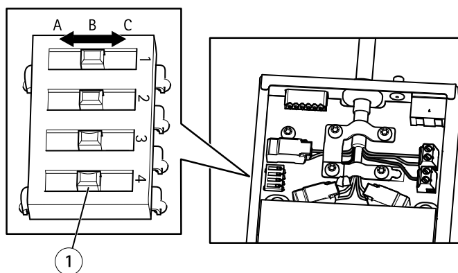
1 Dip switch (4)
