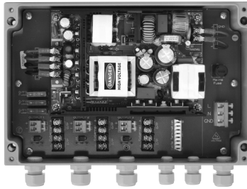
PSU-VAR-150W-3 (x-large)
