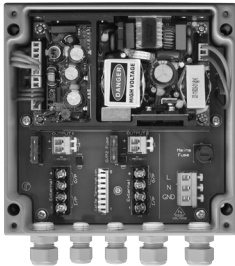
PSU-VAR-100W-2 (large)
